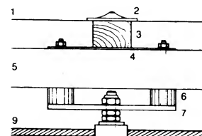
1 roof skin PVC coated polyester fabric 2 BST disks 3 batten: 40 · 60 mm 4 connecting beam 5 batten: 60 · 60 mm 6 plastic spacer h = 25 mm 7 flat steel plate 300/60 · 8 8 pressure clamp 9 wire netting (11.5 mm) 10 bolt
